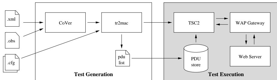
Fig. 5. Overview of the setup used for testing the WAP gateway.
