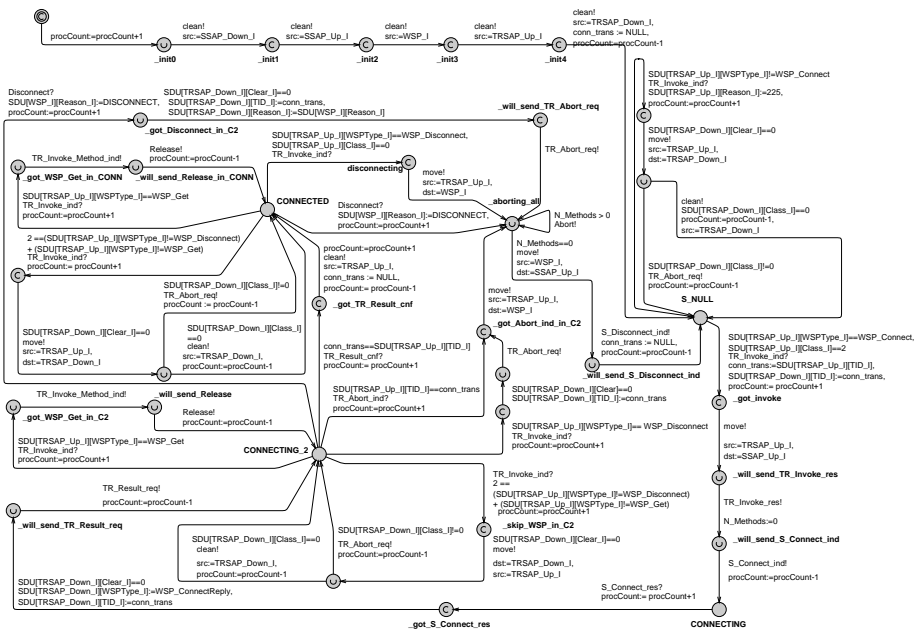
Fig. 12. The Session Manager automaton.
