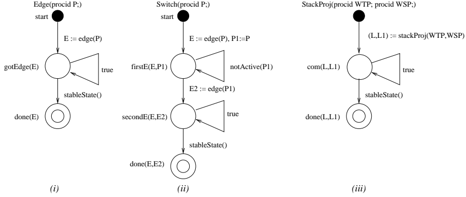
Fig. 6. The three observers used in the case study.
